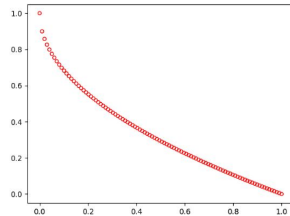
(b) True Pareto front of ZDT1
