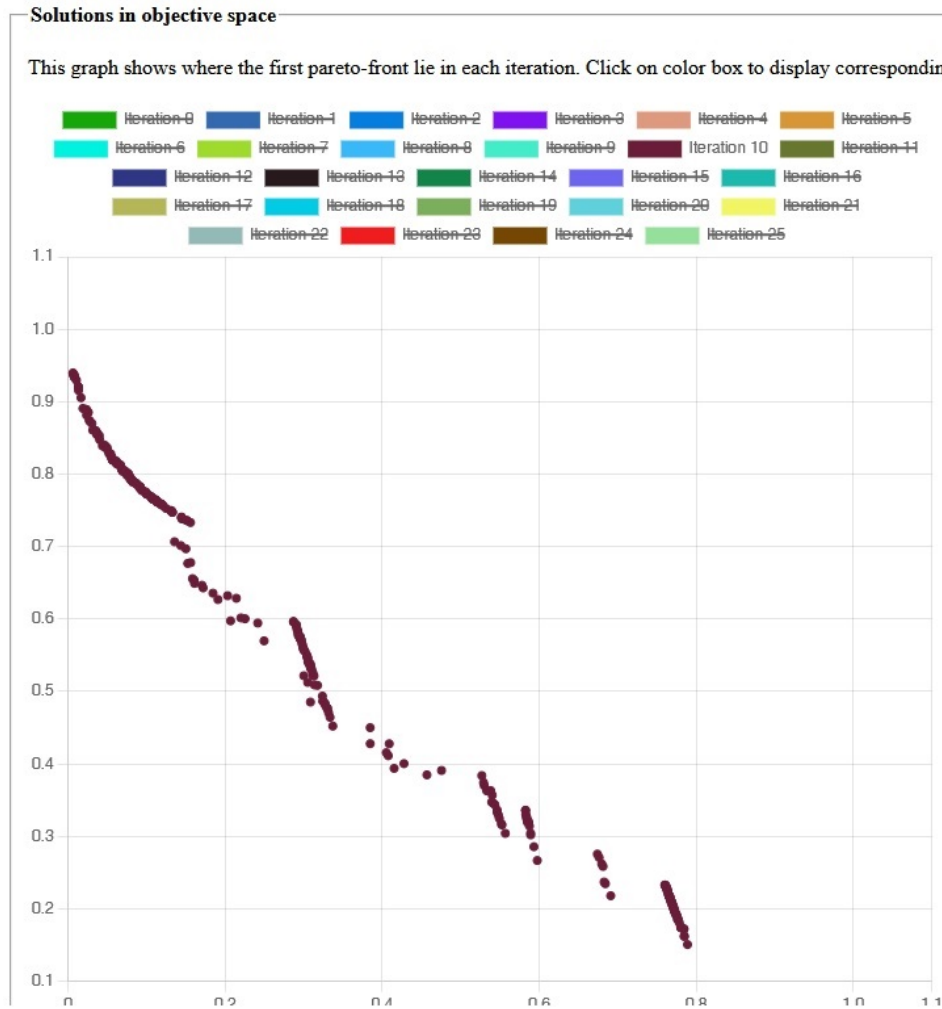
Figure 4.4: Objective values in objective space
