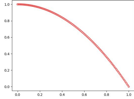
(b) True Pareto front of ZDT2
