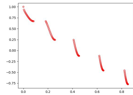
(b) True Pareto front of ZDT3
