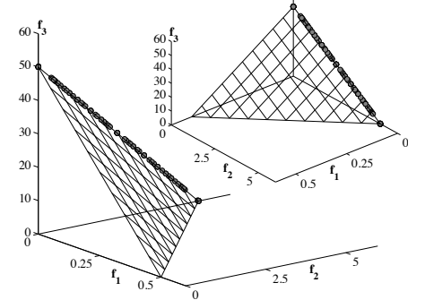
Fig. 26. Obtained solutions by MOEA/D-TCH for scaled DTLZ1.
