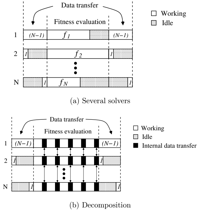
Fig. 13.2. Necessary calculation time of several solvers and decomposition.
