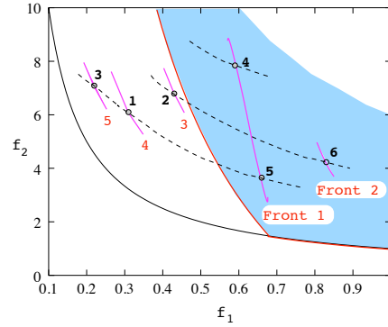
Fig. 3.10. Non-constrained-domination fronts.
