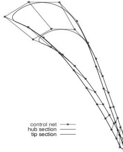
Fig. 11.1. Three-dimensional representation of a blade using B-splines.
