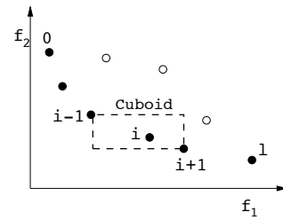
Fig. 3.5. The crowding distance calculation.
