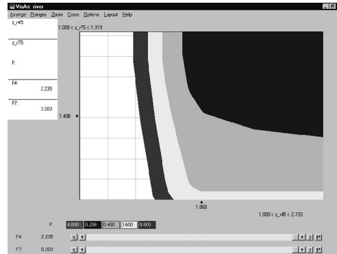
Fig. 9.5. Gray scale copy of a decision map and two scroll-bars.
