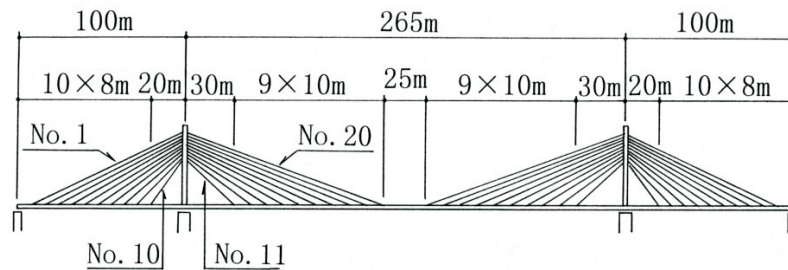
Fig. 10.9. Cable-stayed bridge
