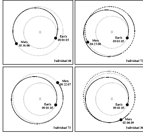
Fig. 3.9. Four trade-off trajectories.
