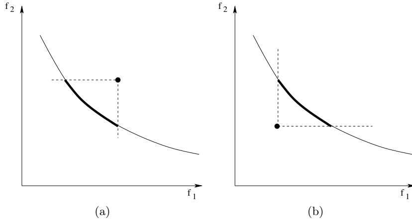
Fig. 6.4. Part of the Pareto optimal front that remains optimal with a given reference point \mathbf{r} and the preference relation from Fonseca and Fleming (1993). The left panel (a) shows a reachable reference point, while the right panel (b) shows an unreachable one. Minimization of objectives is assumed.
