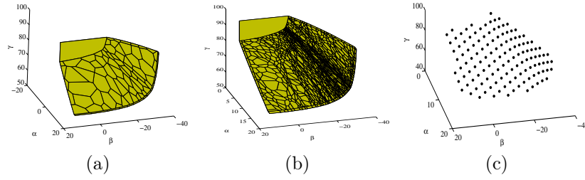
Fig. 11.10. \varepsilon -nondominated set with \varepsilon = 0.1 (a) and \varepsilon = 0.005 (b) and set of representative nondominated points (c).
