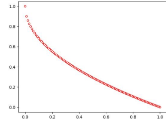
(b) True Pareto front of ZDT1
