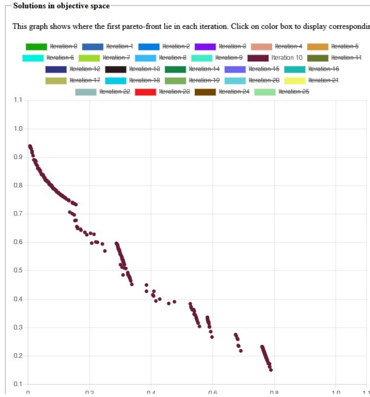
Figure 4.4: Objective values in objective space
