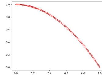
(b) True Pareto front of ZDT2
