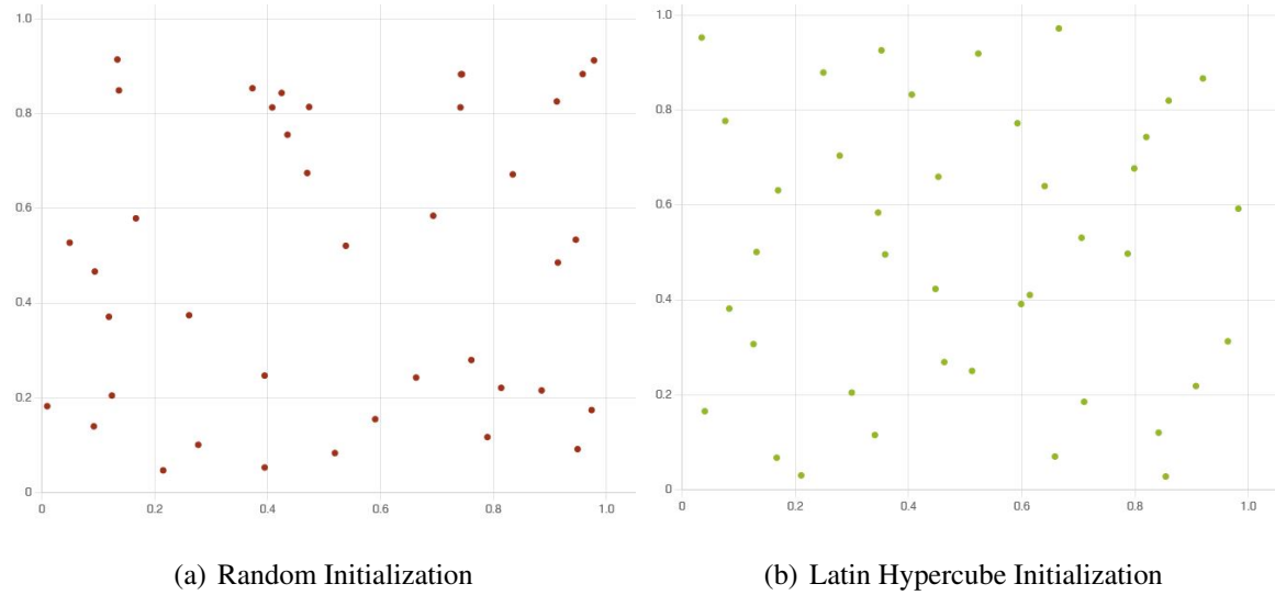
Figure 3.2: Random Sampling vs Latin Hypercube Sampling
