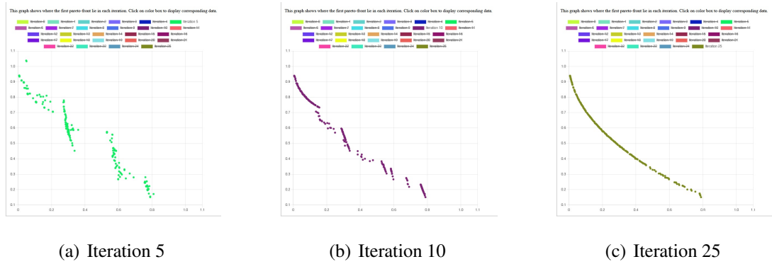
Figure 4.5: Progression of Pareto-Front
